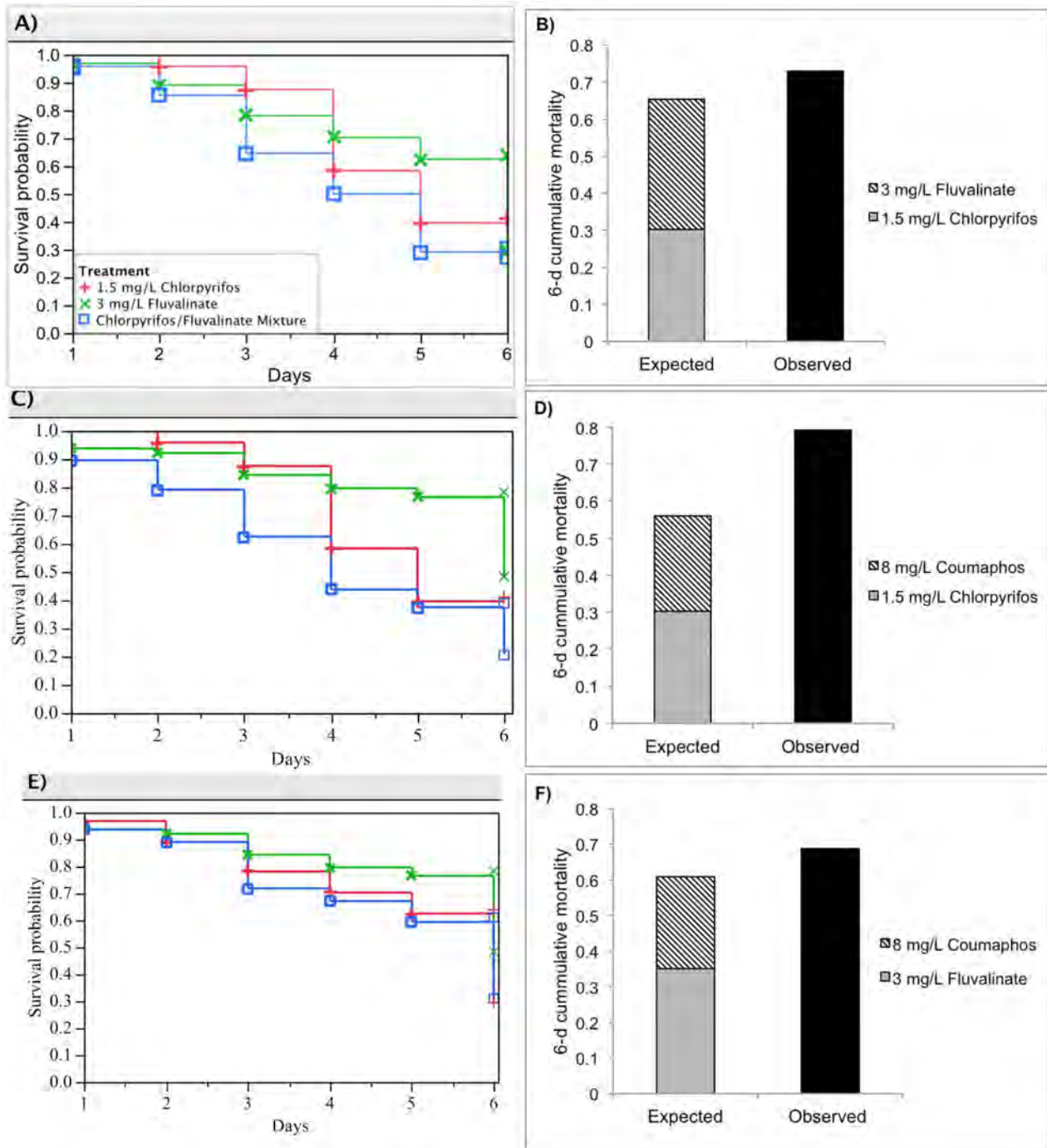
Figure 3. Additive effects for three pairs of pesticide mixtures: 3 mg/L Fluralinate, 1.5 mg/L Chlorpyrifos and the mixture; 8 mg/L Coumaphos, 1.5 mg/L Chlorpyrifos and the mixture; 8 mg/L Coumaphos, 3 mg/L Fluralinate and the mixture. (A), (C) and (E) show the respective Kaplan-Meier survival plots for honey bee larvae reared for each pair of pesticide mixture; (B), (D) and (F) illustrate the interaction determination based on the deviation of observed mixture toxicity (black bar) from the expected additive toxicity (stacked bar). doi:10.1371/journal.pone.0077547.g003
