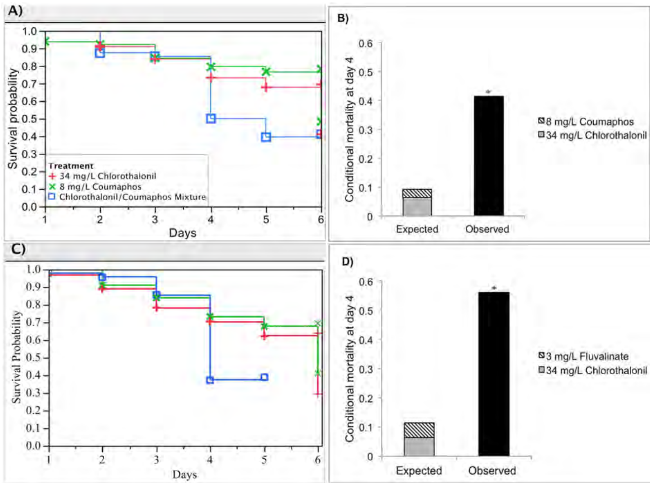
Figure 2. Synergistic interactions for two pairs of pesticide mixtures: 8 mg/L Coumaphos, 34 mg/L Chlorothalonil and the mixture; 3 mg/L Fluvinate, 34 mg/L Chlorothalonil and the mixture. (A) and (C) show the respective Kaplan-Meier survival plots for honey bee larvae reared for each pair of pesticide mixture; (B) and (D) illustrate the interaction determination based on the deviation of observed mixture toxicity (black bar) from the expected additive toxicity (stacked bar). Asterisks denote significant difference from the expected additive toxicity (Mann-Whitney test, p < 0.0001 ). doi:10.1371/journal.pone.0077547.g002
